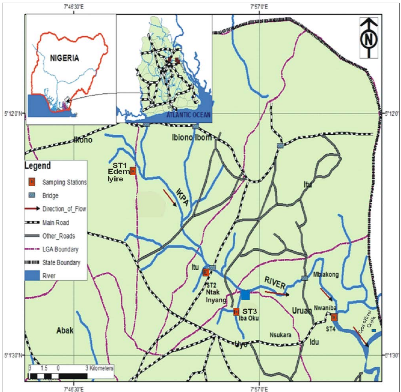
a. Location of Ikpa River on the Map of Akwa Ibom State b. Location of Akwa Ibom State on the Map of Nigeria
